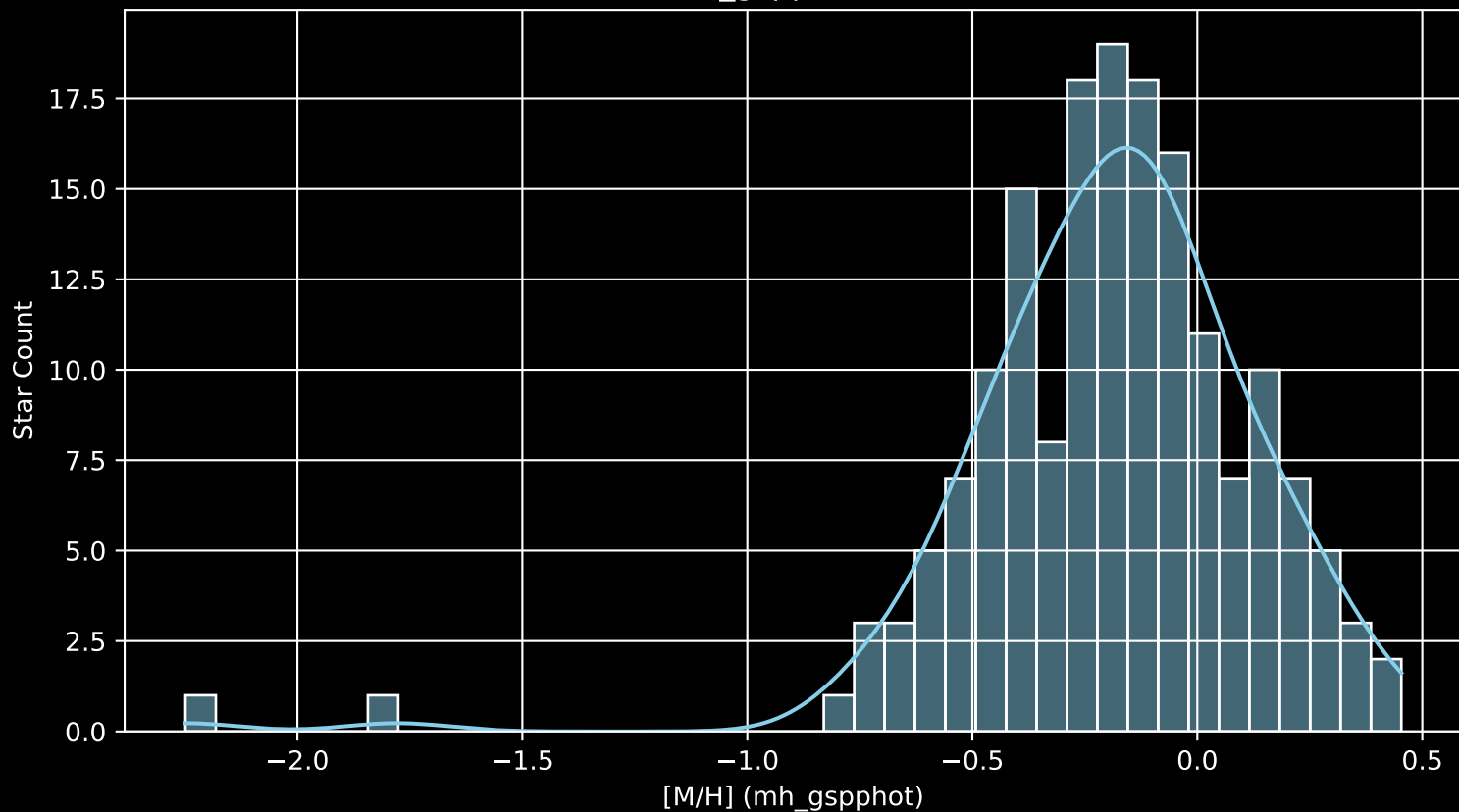
APOGEE DR17 Field: [263-30-O TESS [M/H] (mh_gspphot) (n= 170)
