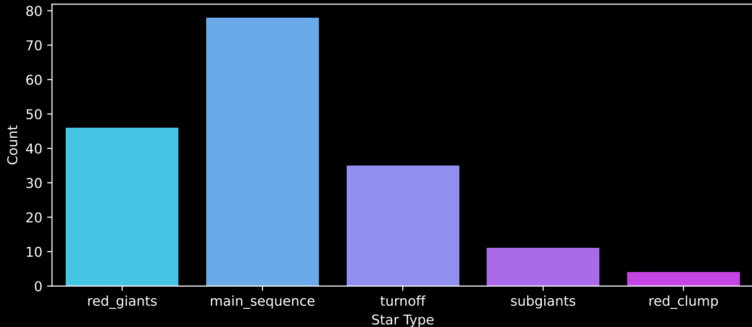
APOGEE DR17 Field: [263-30-O_TESS] Count plot of Star Type
