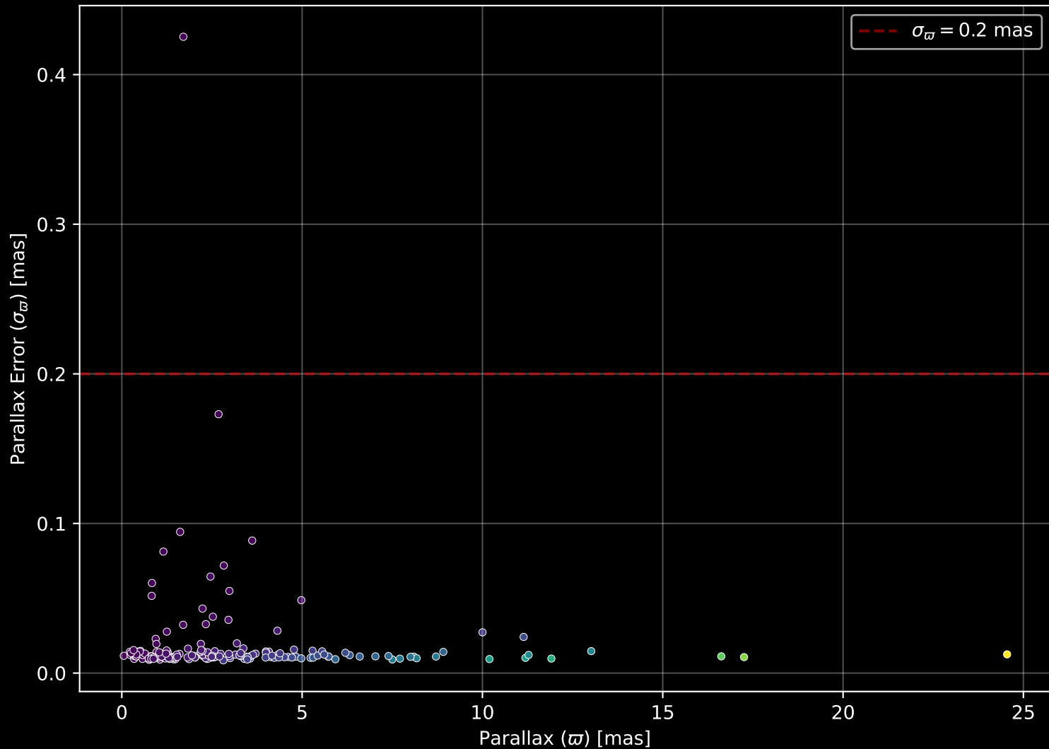
APOGEE DR17 Field: [263-30-O_TESS] Parallax Quality (n= 174)
