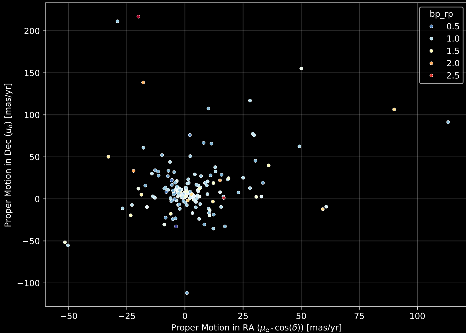
APOGEE DR17 Field: [263-30-O_TESS] Proper Motion Diagram (n= 174)
