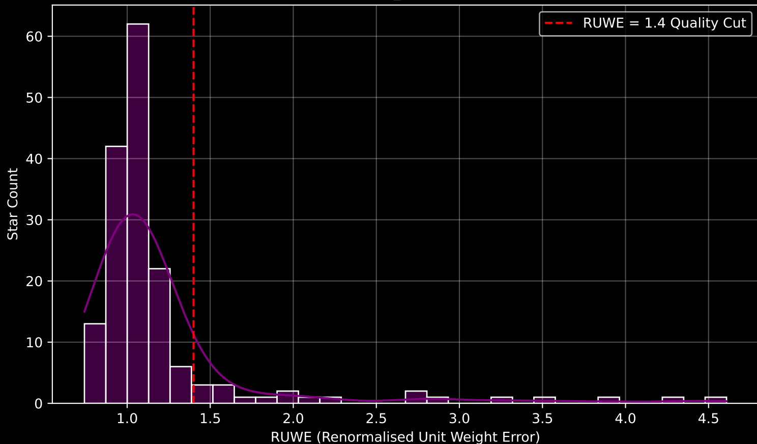
GAPOGEE DR17 Field [263-30-O_TESS] RUWE Distribution (n= 165)
