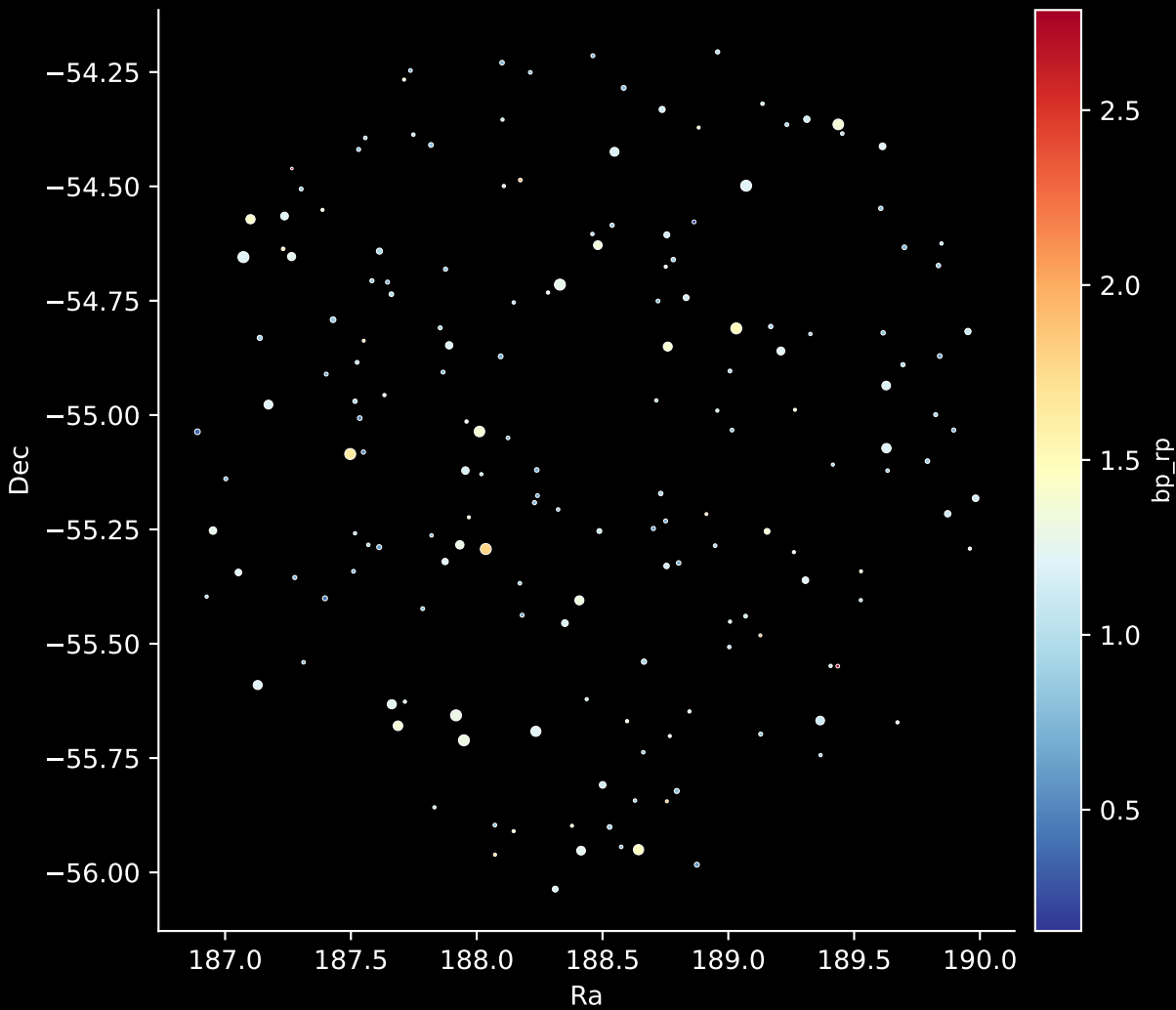
APOGEE DR17 Field: [263-30-O_TESS] Stars: 174
